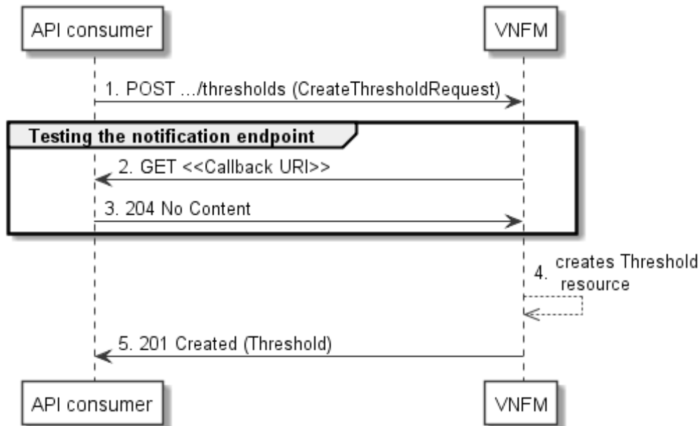
Figure 6.3.5-1: Flow of threshold creation
